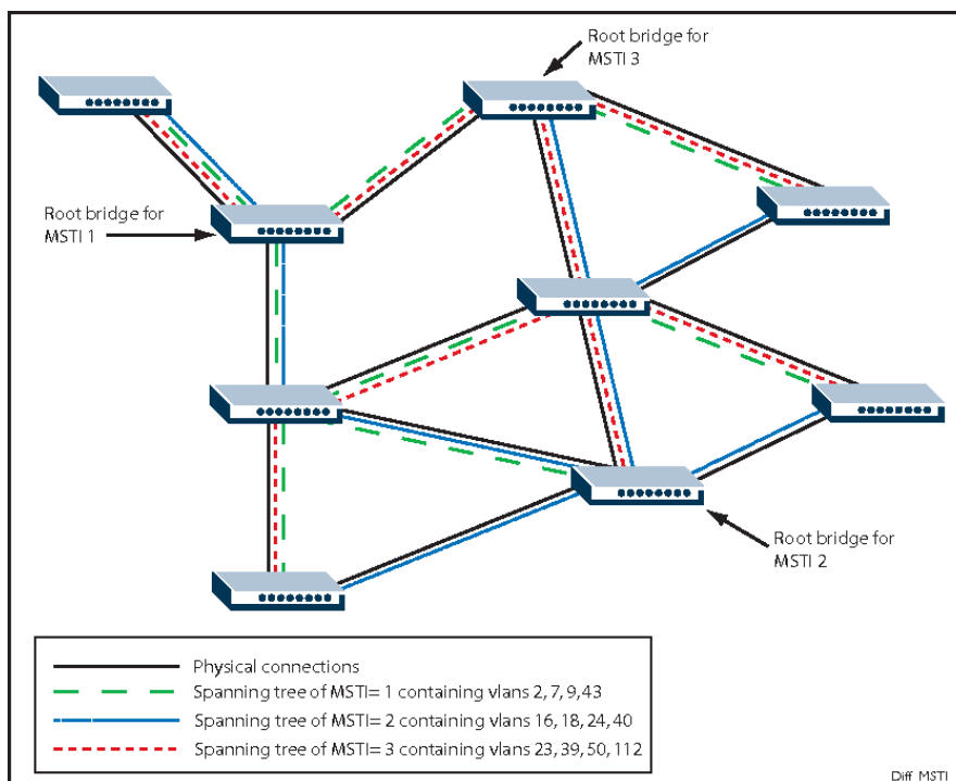
Fig. 39 Example MSTI Configuration
