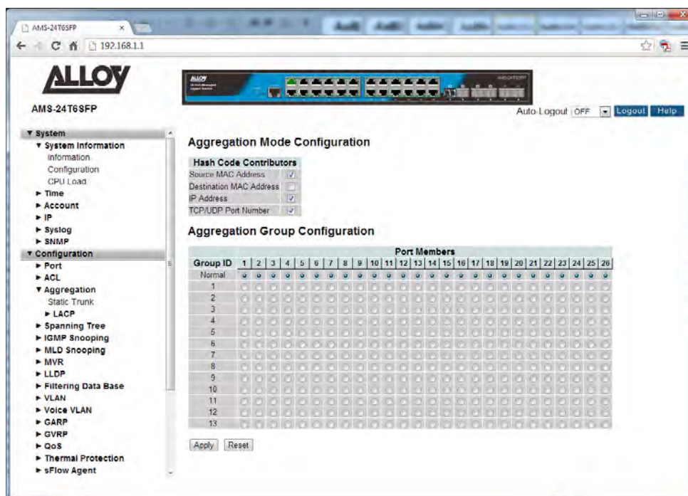
Fig. 32 Configuring a static trunk group
